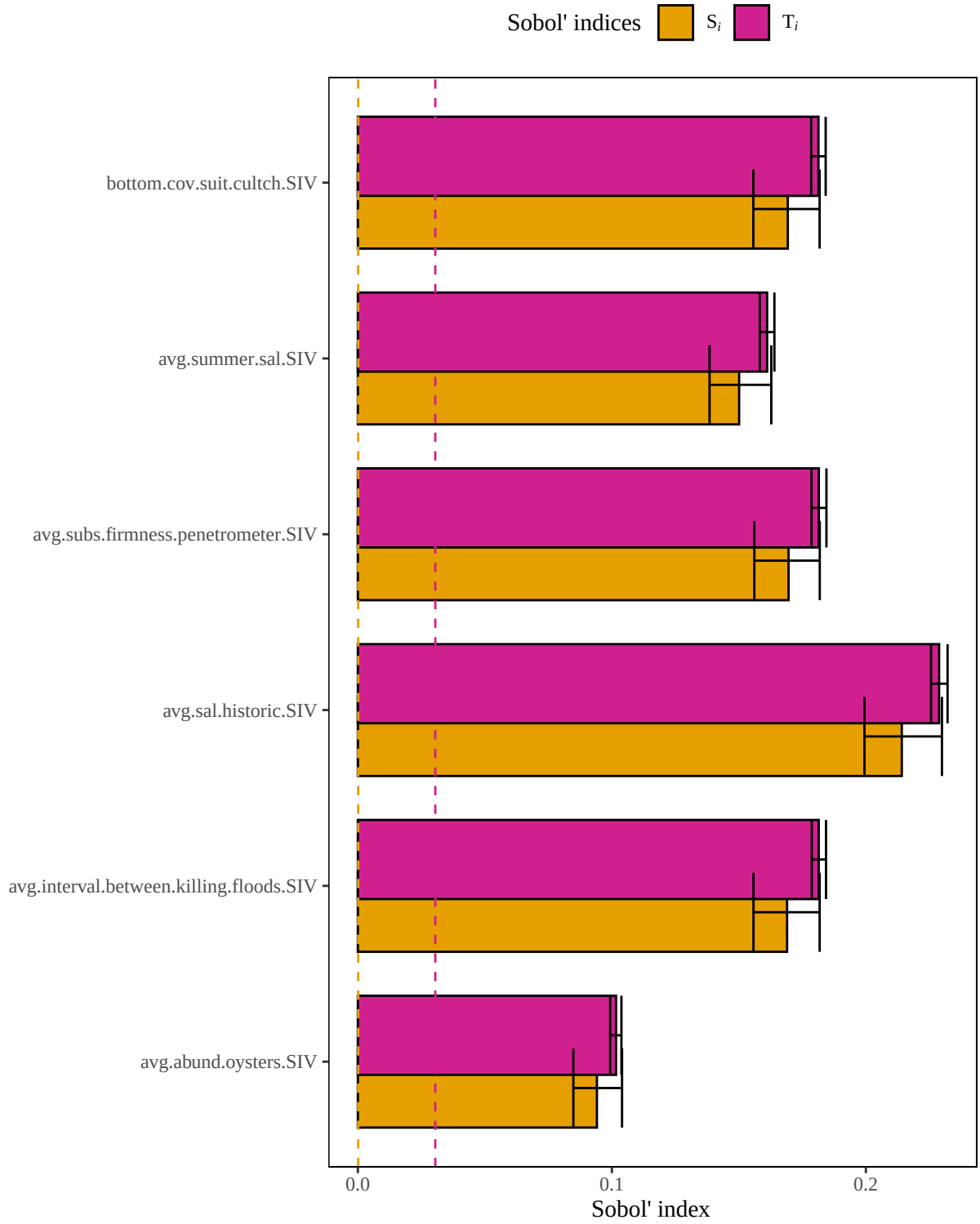
Figure 5. Results of a sensitivity analysis for the americanoysterGulfofMexTypical model based on a geometric mean structure. Dashed lines represent baseline numerical approximation error for S_i and T_i ( i.e. , dummy variables).
